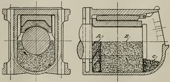
FIG. 1. METHOD OF PACKING JOURNAL BOXES
